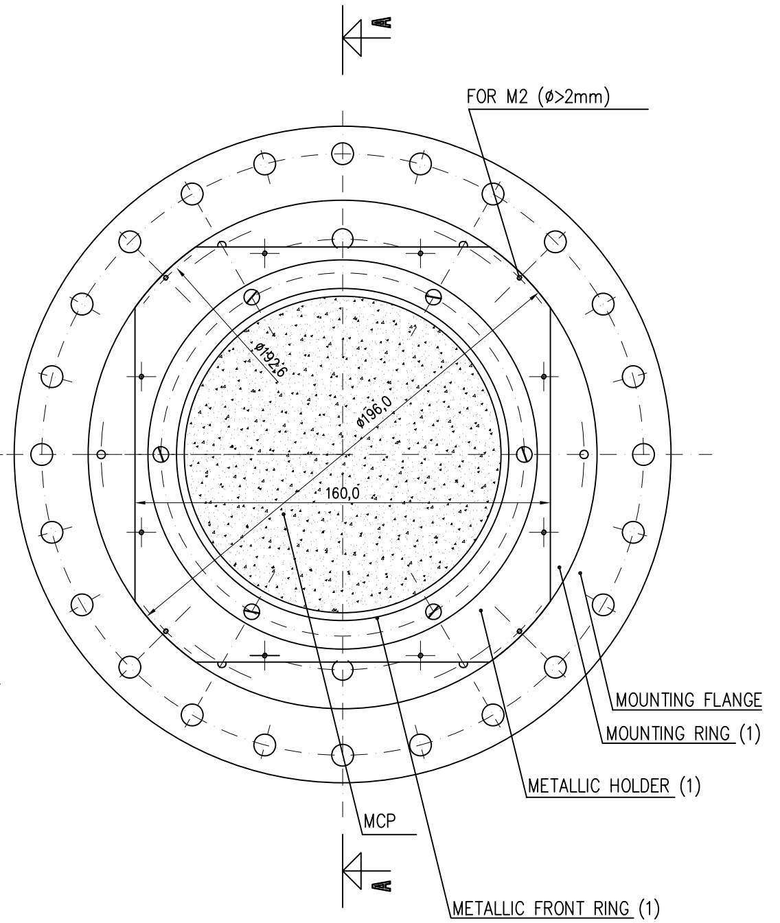
TOP VIEW
